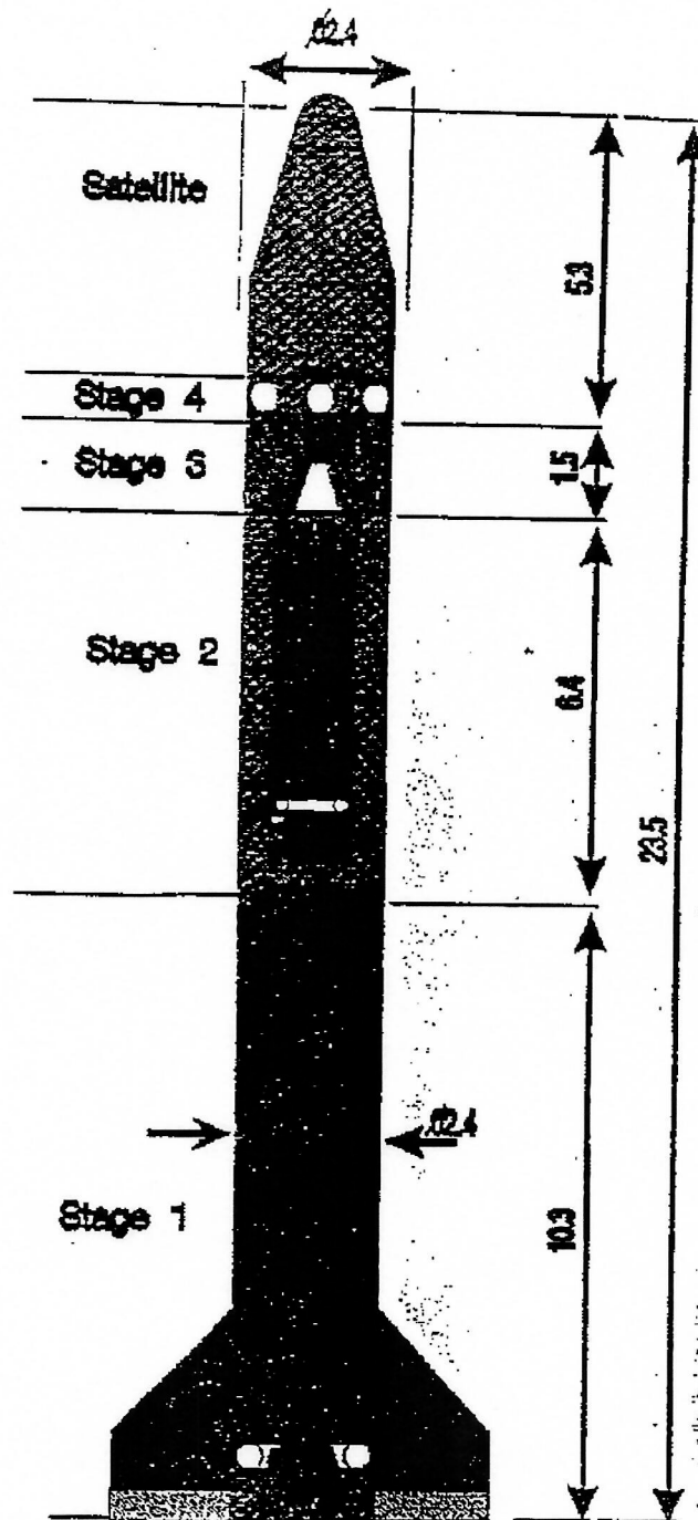
Figure 2.1: RSA4 LAUNCH VEHICLE
